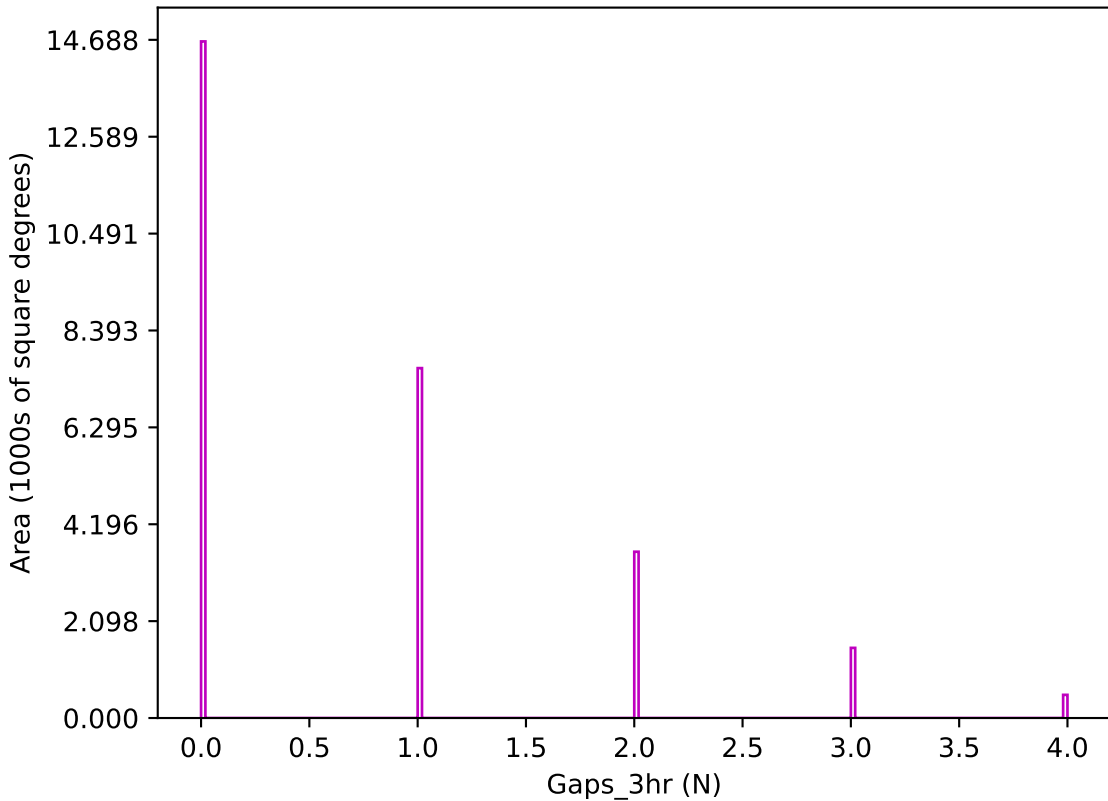
weather_cloudso2v3.4_10yrs z band: Gaps_3hr
