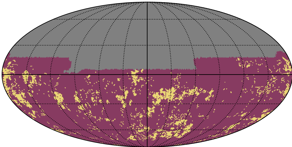
weather_cloudso2v3.4_10yrs u band: Gaps_3hr
