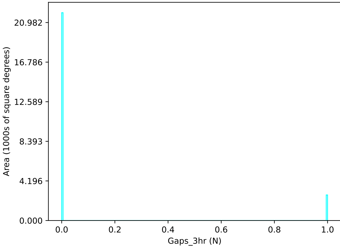
weather_cloudso2v3.4_10yrs u band: Gaps_3hr
