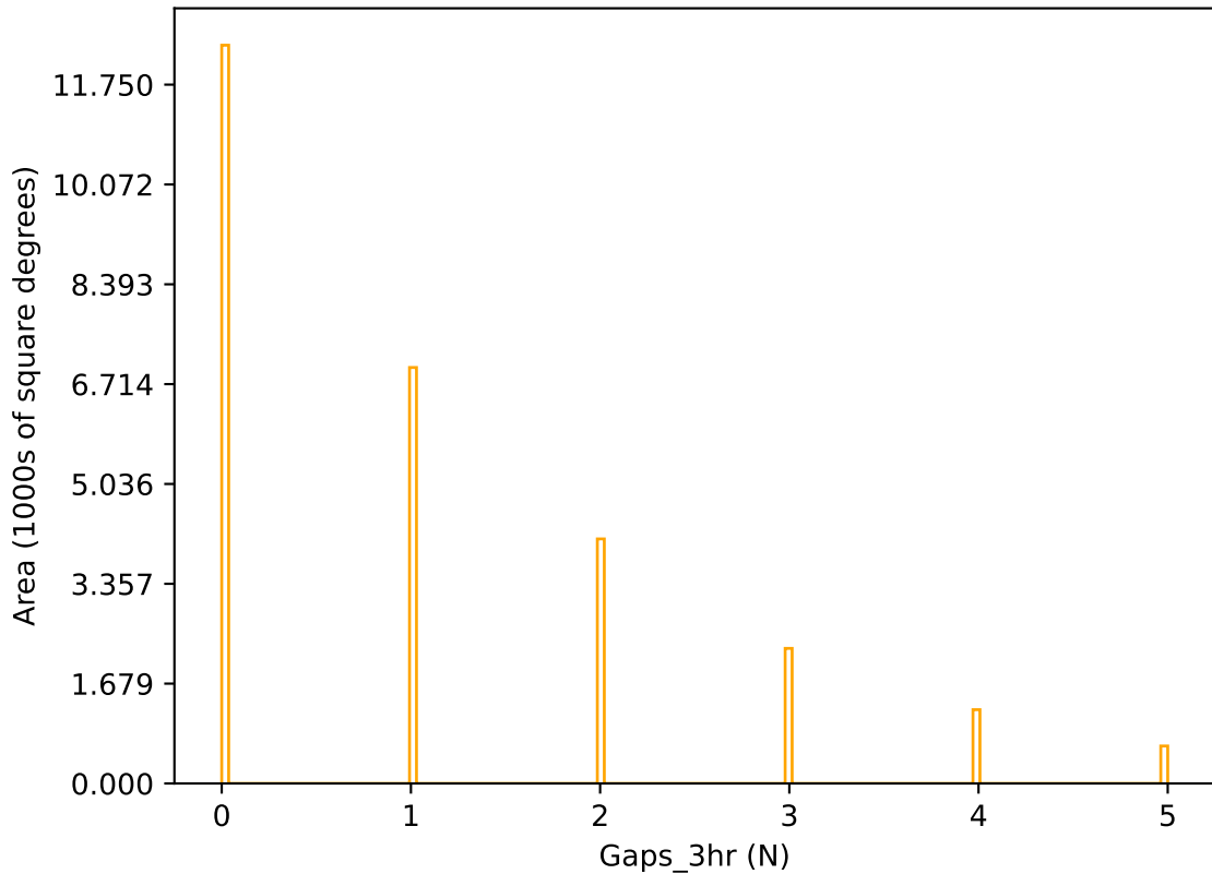
weather_cloudso2v3.4_10yrs r band: Gaps_3hr
