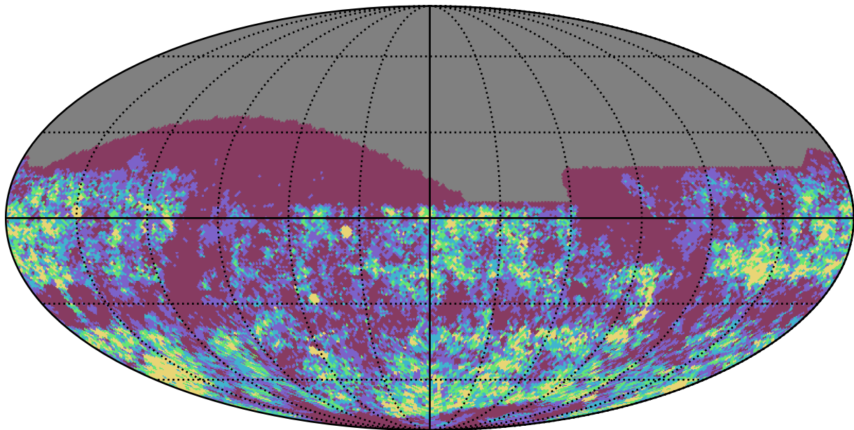
weather_cloudso2v3.4_10yrs i band: Gaps_3hr
