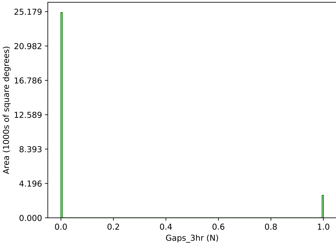
weather_cloudso2v3.4_10yrs g band: Gaps_3hr
