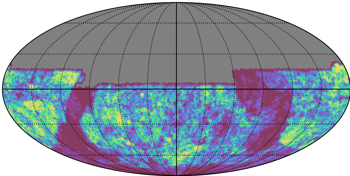
weather_cloudso2v3.4_10yrs u band: Gaps_24hr
