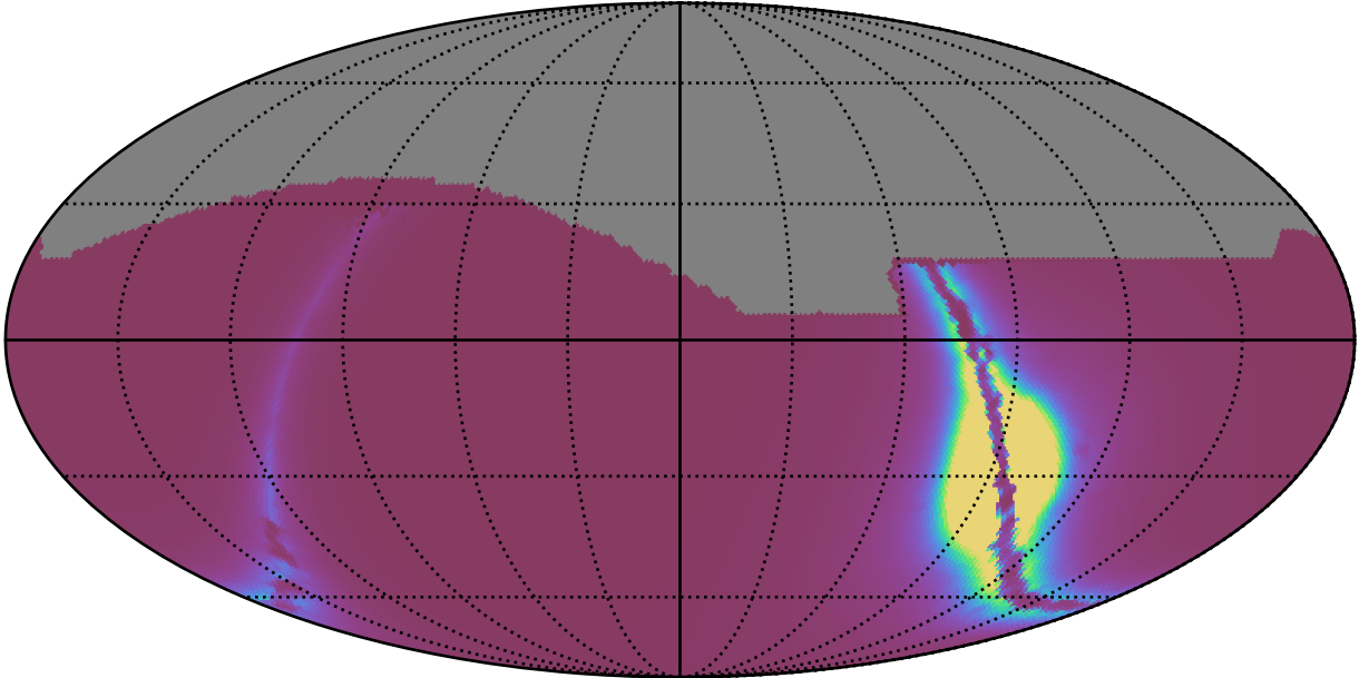
weather_cloudso2v3.4_10yrs : GalplaneFootprintMetric_xray_binaries_map_Tau_73_0
