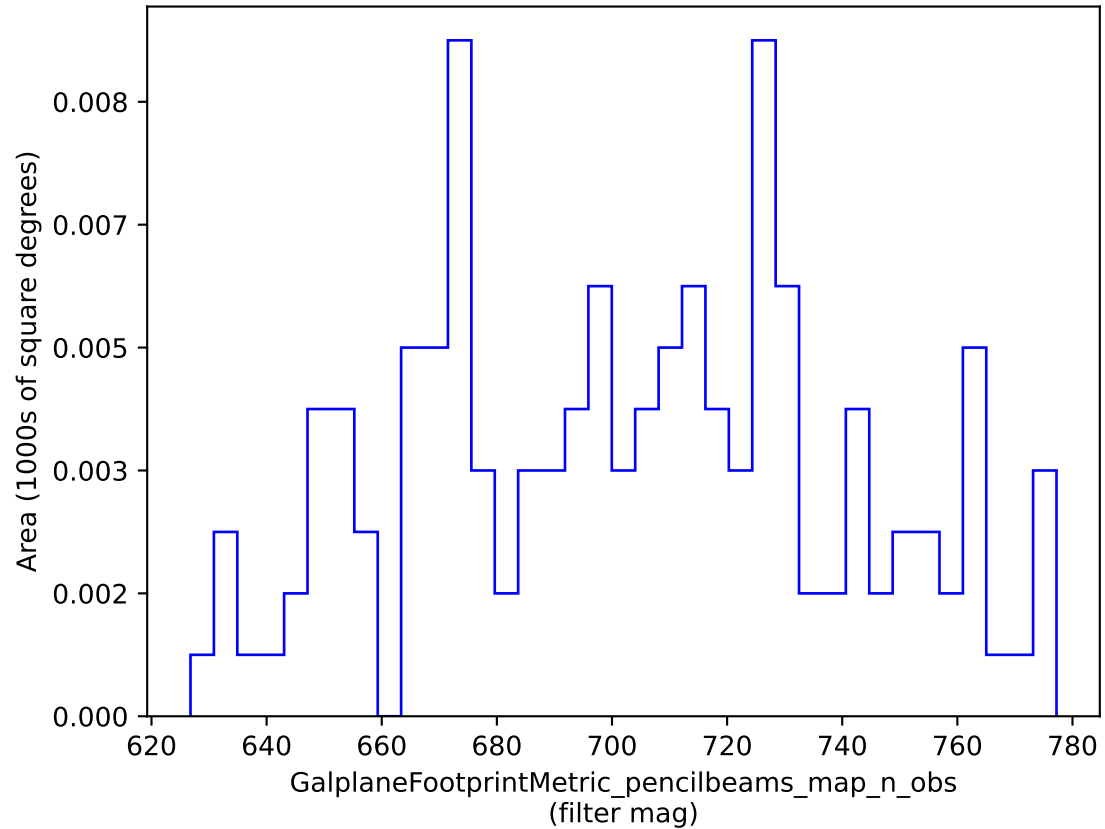
weather_cloudso2v3.4_10yrs : GalplaneFootprintMetric_pencilbeams_map_n_obs
