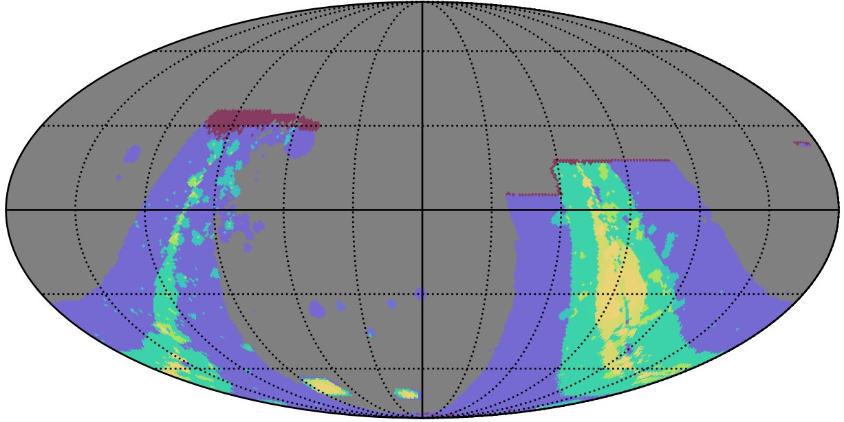
weather_cloudso2v3.4_10yrs : GalplaneFootprintMetric_combined_map_Tau_73_0
