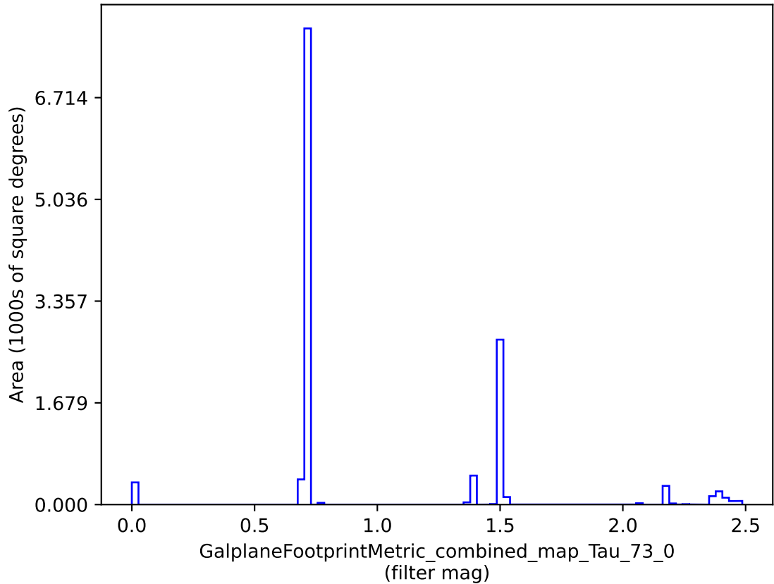
weather_cloudso2v3.4_10yrs : GalplaneFootprintMetric_combined_map_Tau_73_0
