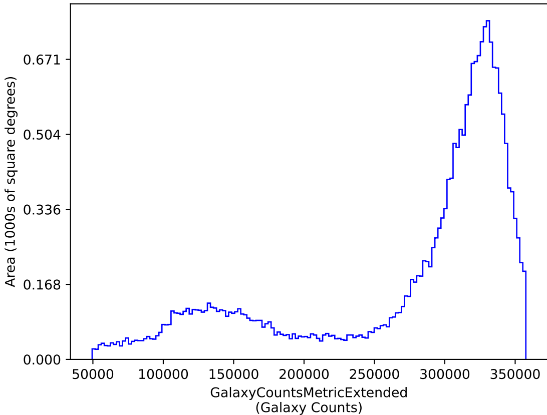
weather_cloudso2v3.4_10yrs y: GalaxyCountsMetricExtended
