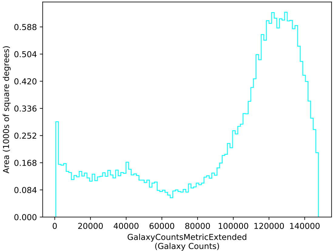
weather_cloudso2v3.4_10yrs u: GalaxyCountsMetricExtended
