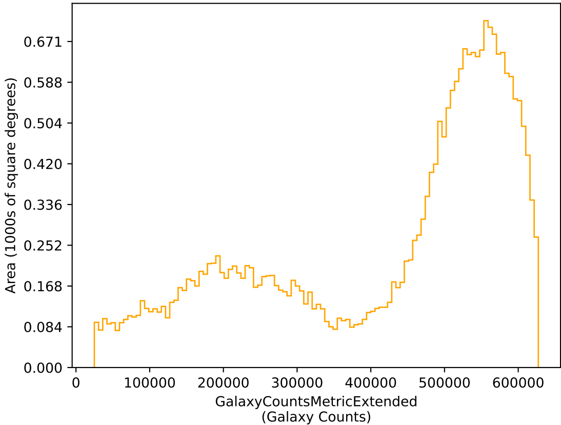
weather_cloudso2v3.4_10yrs r: GalaxyCountsMetricExtended
