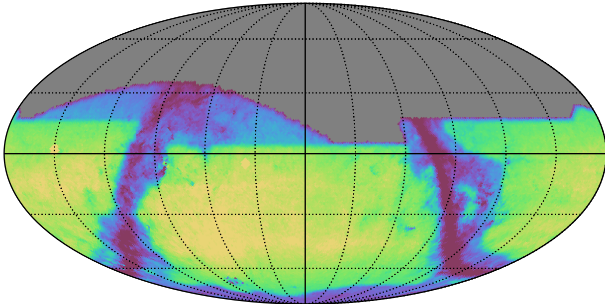
weather_cloudso2v3.4_10yrs i: GalaxyCountsMetricExtended
