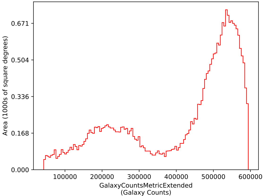
weather_cloudso2v3.4_10yrs i: GalaxyCountsMetricExtended
