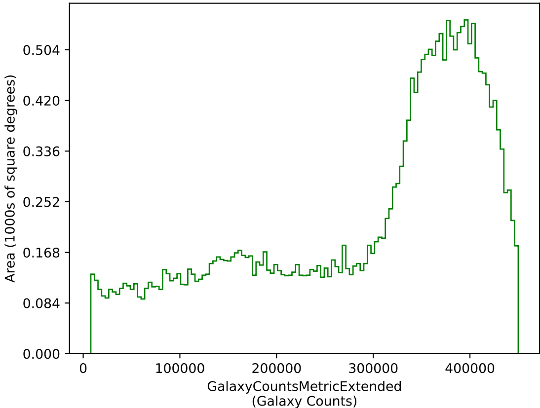
weather_cloudso2v3.4_10yrs g: GalaxyCountsMetricExtended
