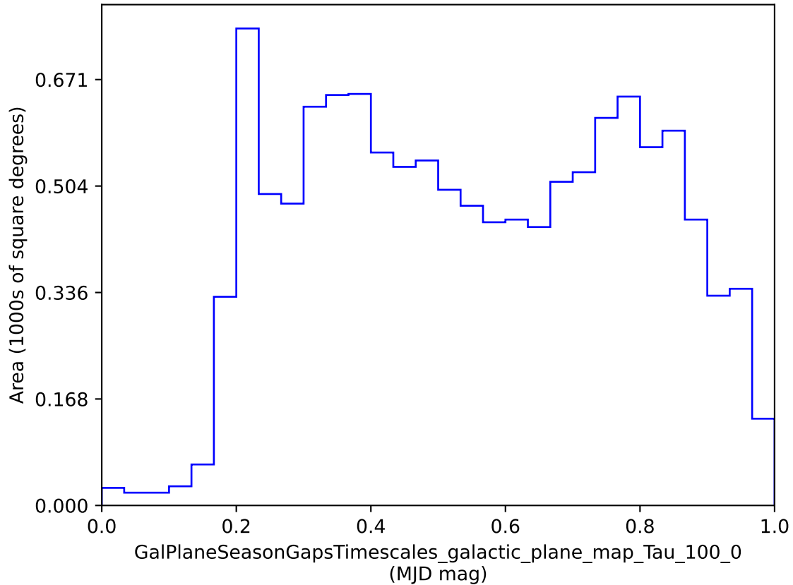
weather_cloudso2v3.4_10yrs : GalPlaneSeasonGapsTimescales_galactic_plane_map_Tau_100_0
