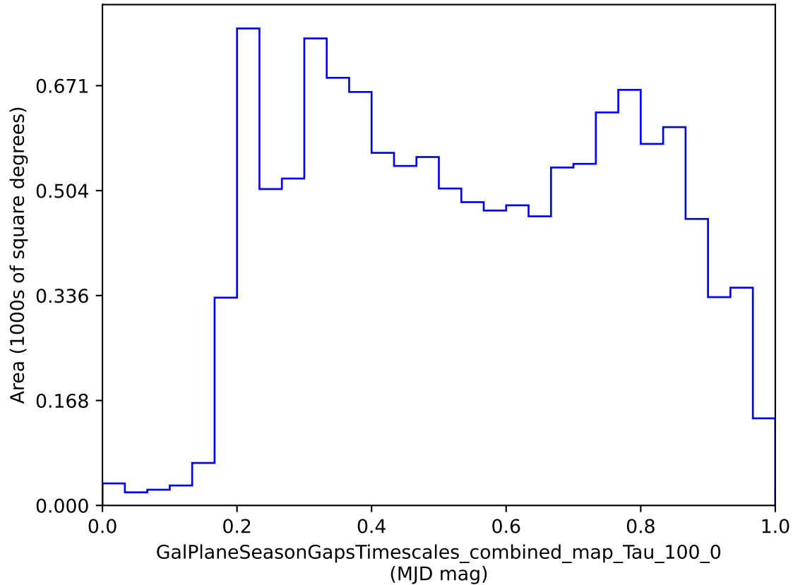
weather_cloudso2v3.4_10yrs : GalPlaneSeasonGapsTimescales_combined_map_Tau_100_0
