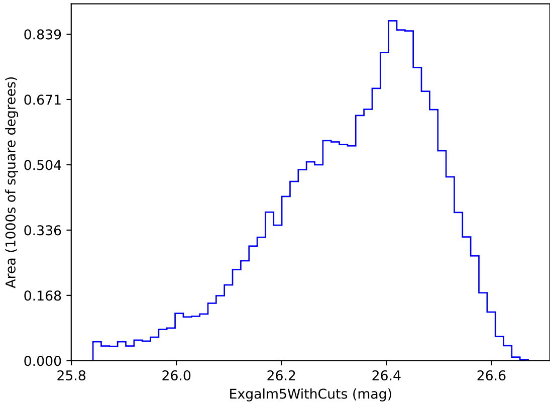
weather_cloudso2v3.4_10yrs i band non-DD year 9: Exgalml5WithCuts
