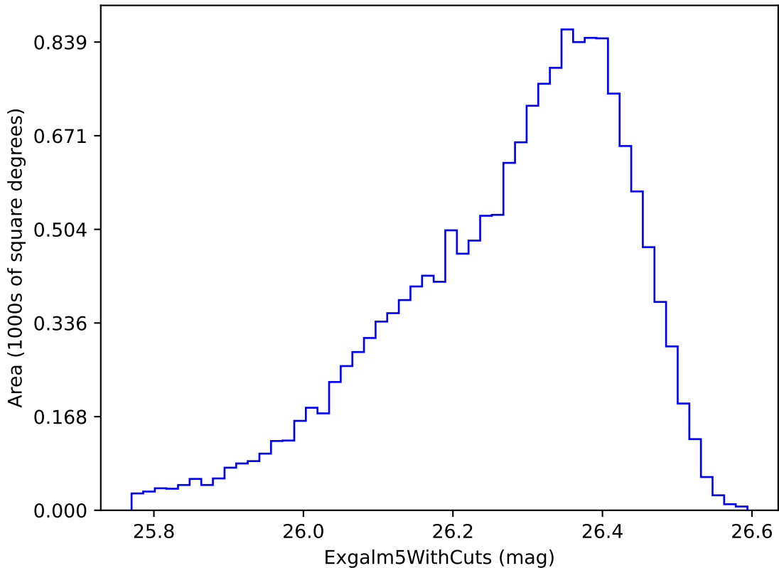
weather_cloudso2v3.4_10yrs i band non-DD year 8: Exgalml5WithCuts
