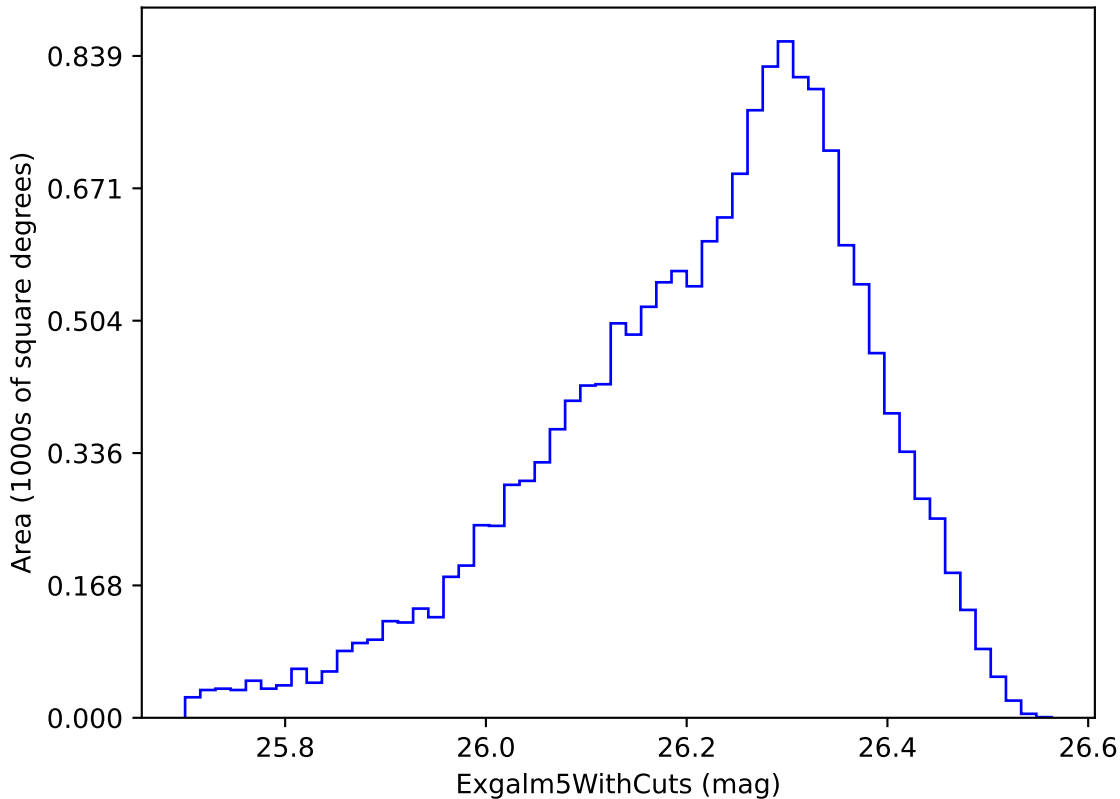
weather_cloudso2v3.4_10yrs i band non-DD year 7: Exgalml5WithCuts
