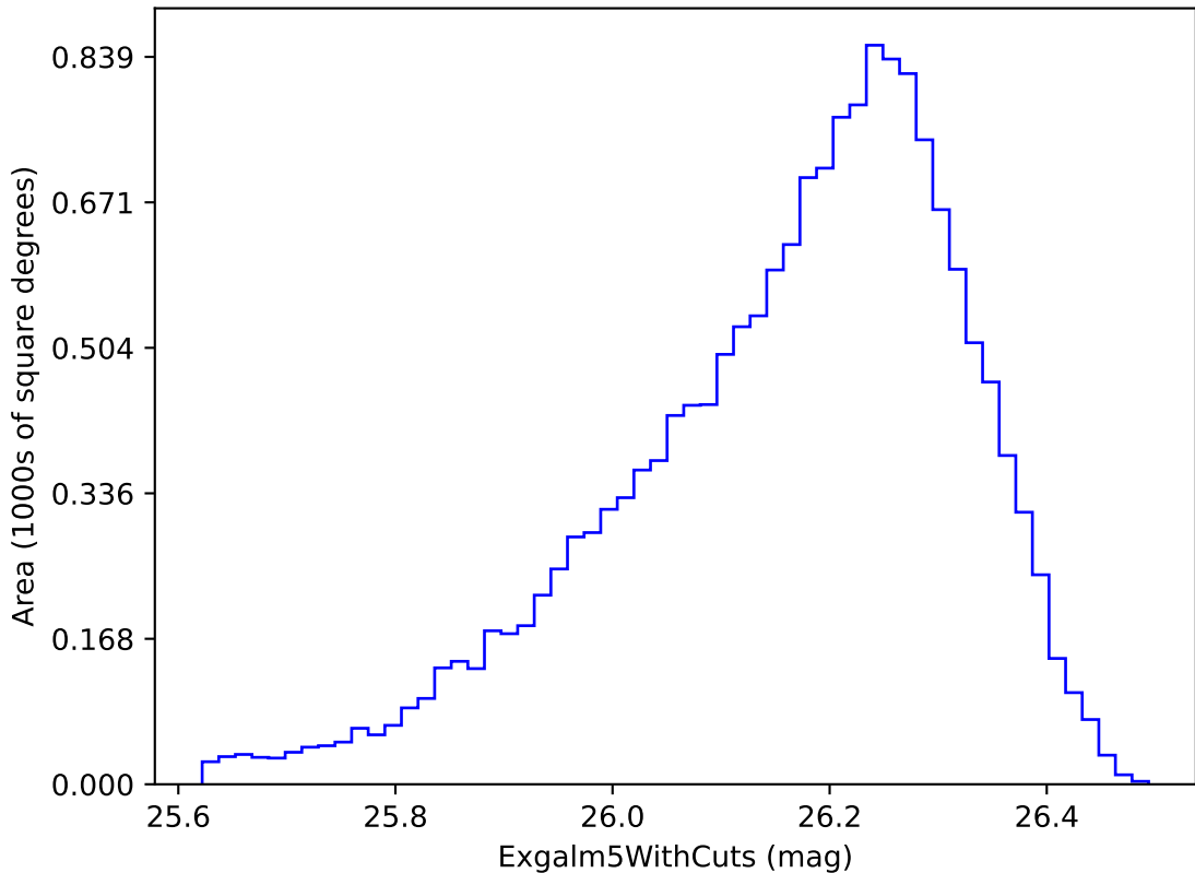
weather_cloudso2v3.4_10yrs i band non-DD year 6: Exgalml5WithCuts
