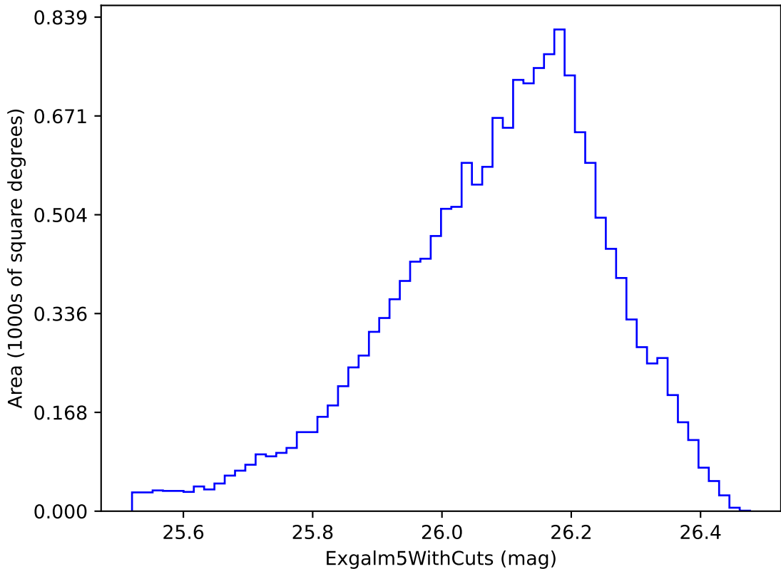
weather_cloudso2v3.4_10yrs i band non-DD year 5: Exgalml5WithCuts
