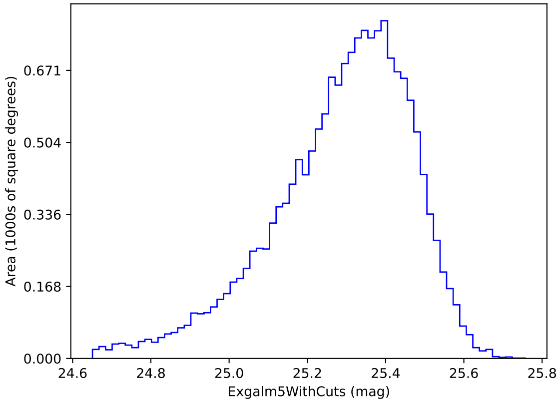
weather_cloudso2v3.4_10yrs i band non-DD year 1: Exgalml5WithCuts
