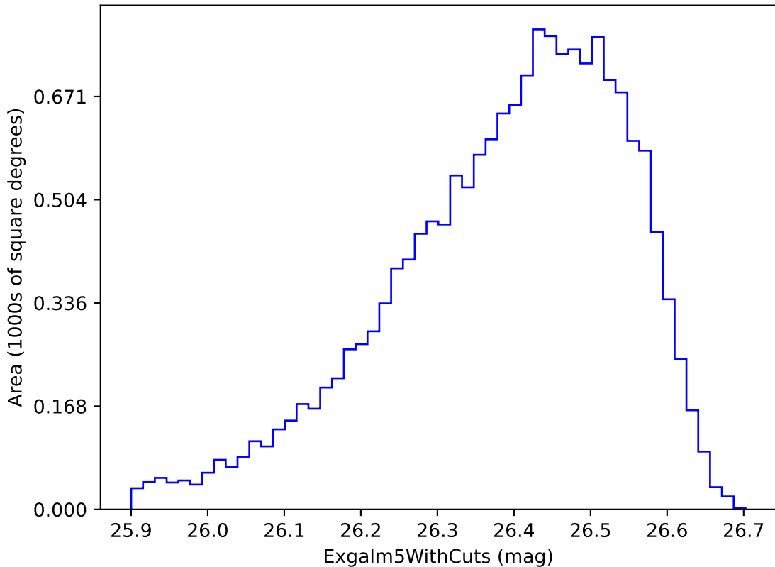
weather_cloudso2v3.4_10yrs i band non-DD year 10: ExgalM5WithCuts
