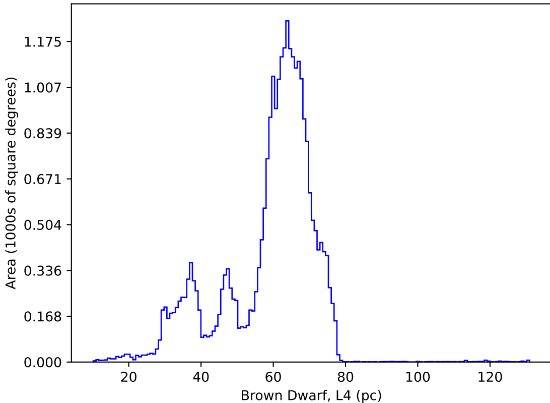
weather_cloudso2v3.4_10yrs : Brown Dwarf, L4
