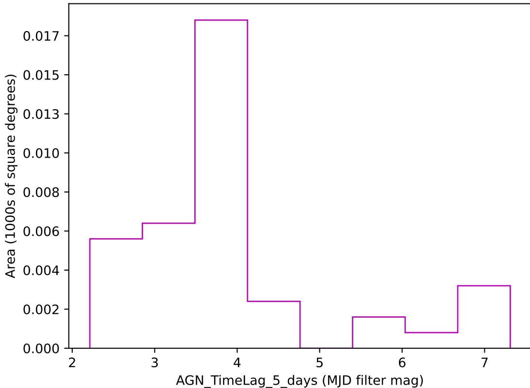
weather_cloudso2v3.4_10yrs z band: AGN_TimeLag_5_days
