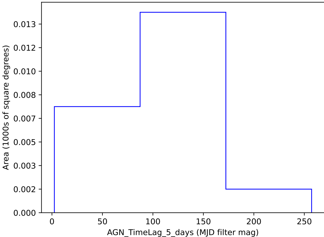
weather_cloudso2v3.4_10yrs y band: AGN_TimeLag_5_days
