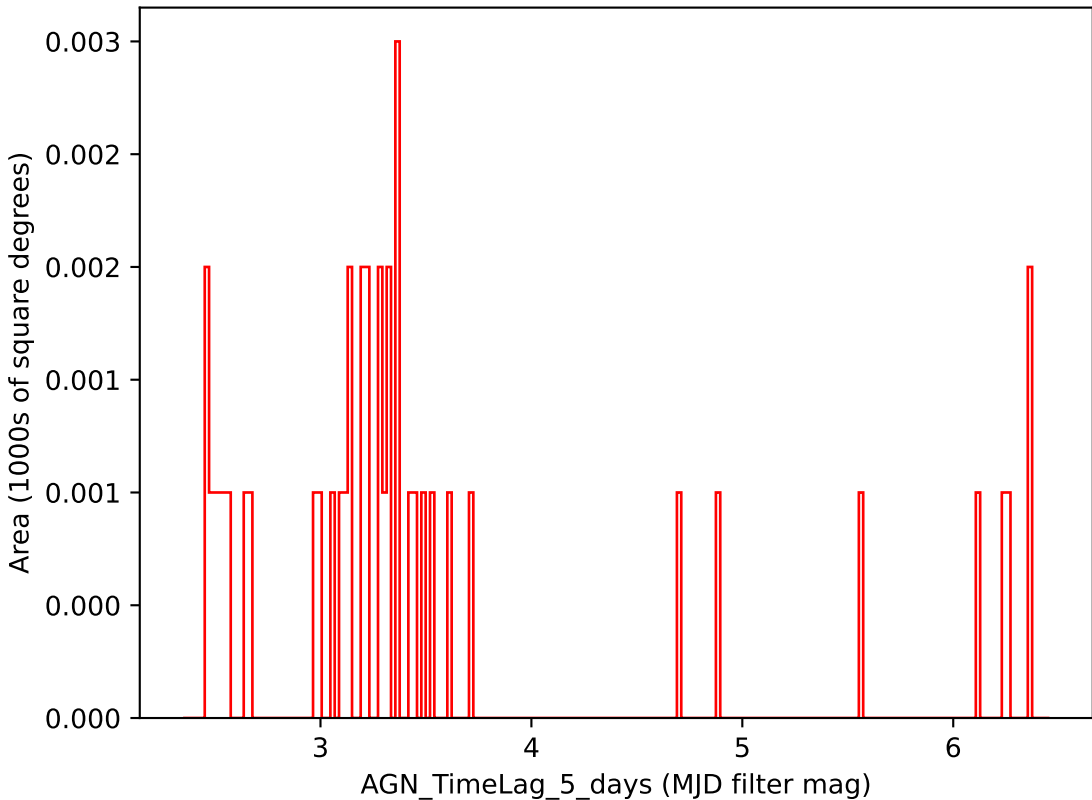
weather_cloudso2v3.4_10yrs i band: AGN_TimeLag_5_days
