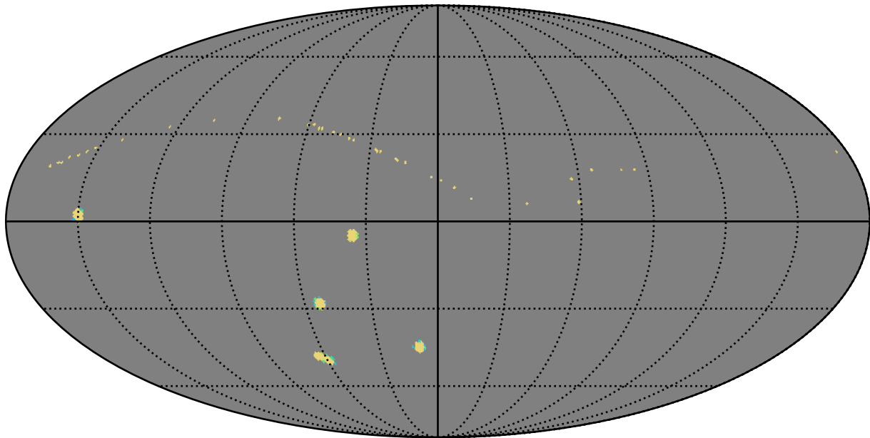
weather_cloudso2v3.4_10yrs all bands: AGN_TimeLag_5_days
