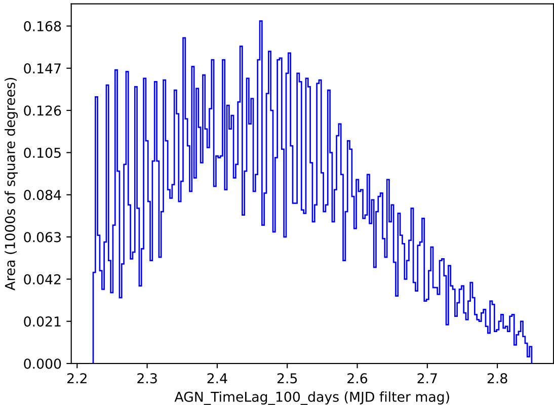
weather_cloudso2v3.4_10yrs y band: AGN_TimeLag_100_days
