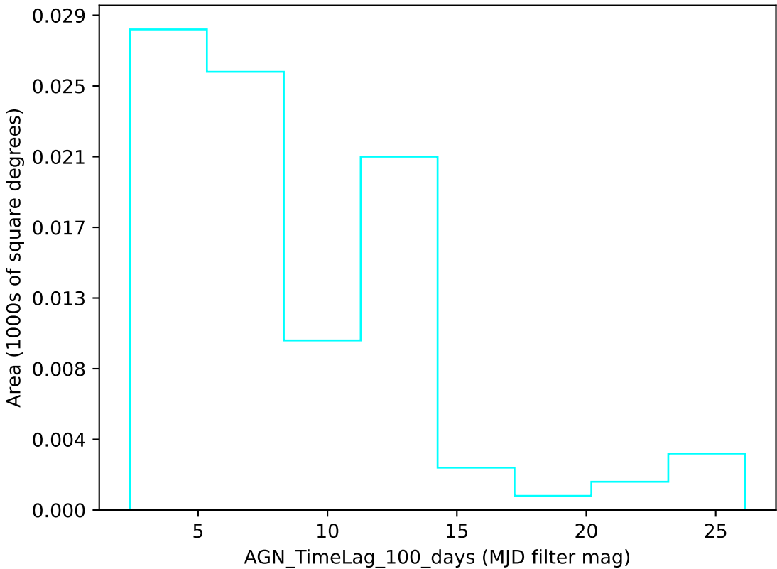
weather_cloudso2v3.4_10yrs u band: AGN_TimeLag_100_days
