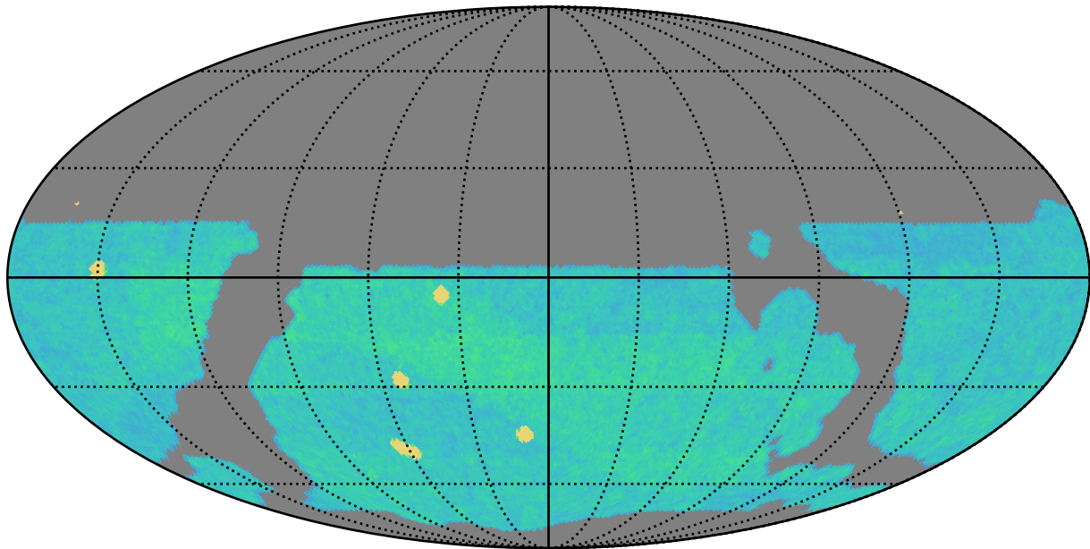
weather_cloudso2v3.4_10yrs i band: AGN_TimeLag_100_days
