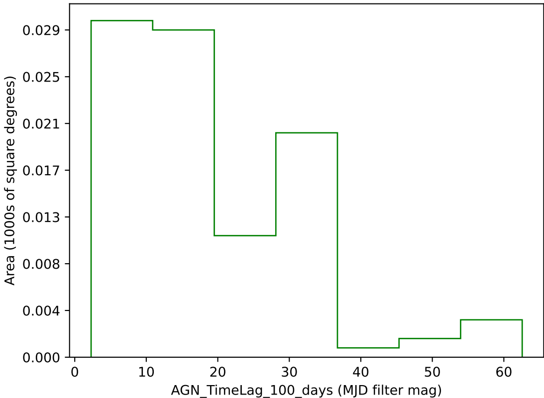
weather_cloudso2v3.4_10yrs g band: AGN_TimeLag_100_days
