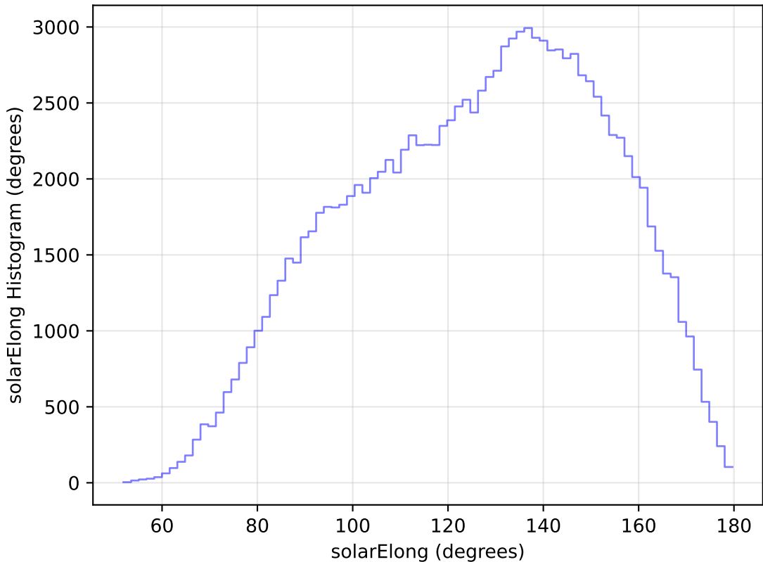
weather_cloudso2v3.4_10yrs WFD u band: solarElong Histogram
