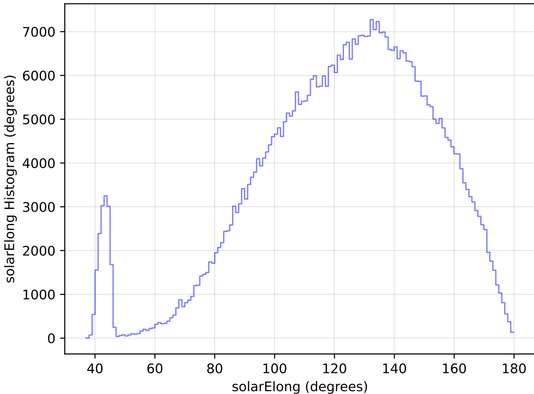
weather_cloudso2v3.4_10yrs WFD r band: solarElong Histogram
