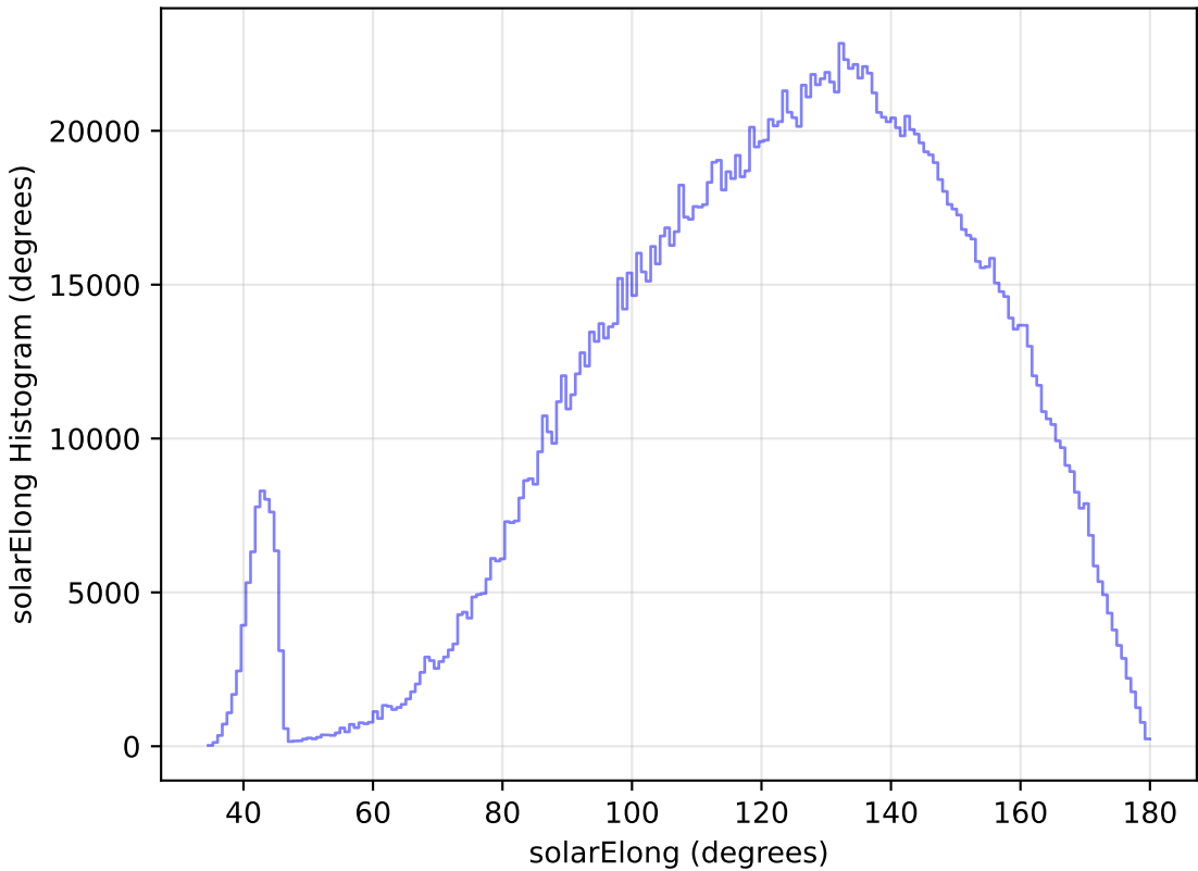
weather_cloudso2v3.4_10yrs WFD all bands: solarElong Histogram
