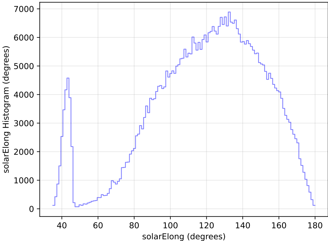
weather_cloudso2v3.4_10yrs All sky z band: solarElong Histogram
