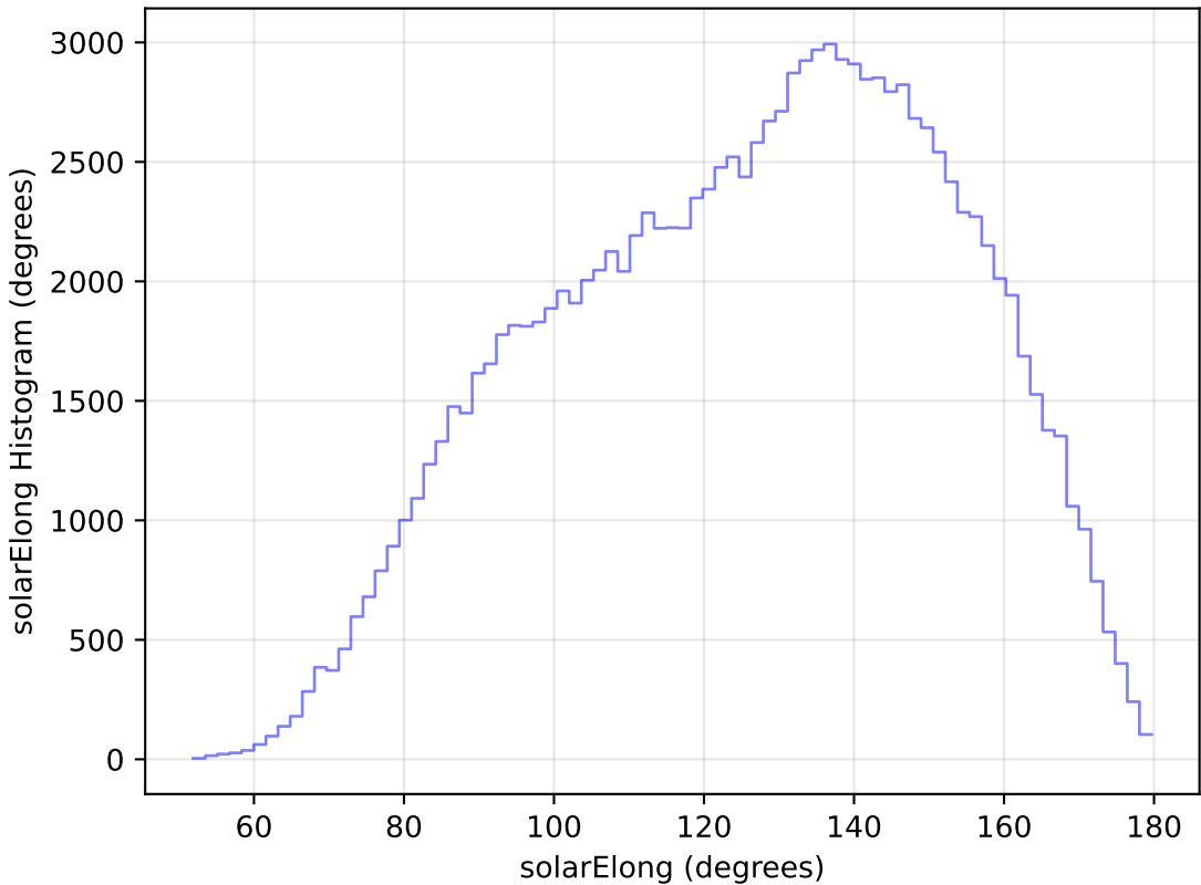
weather_cloudso2v3.4_10yrs All sky u band: solarElong Histogram
