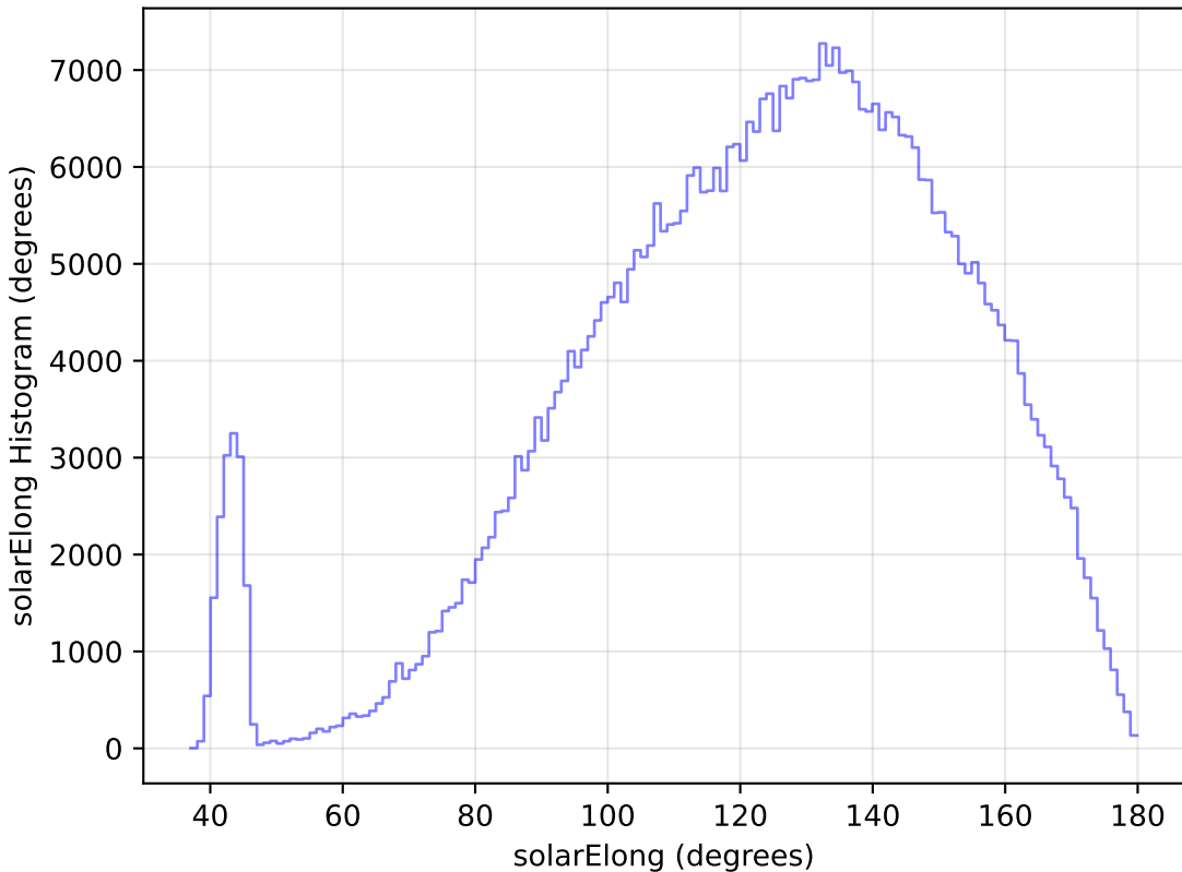
weather_cloudso2v3.4_10yrs All sky r band: solarElong Histogram
