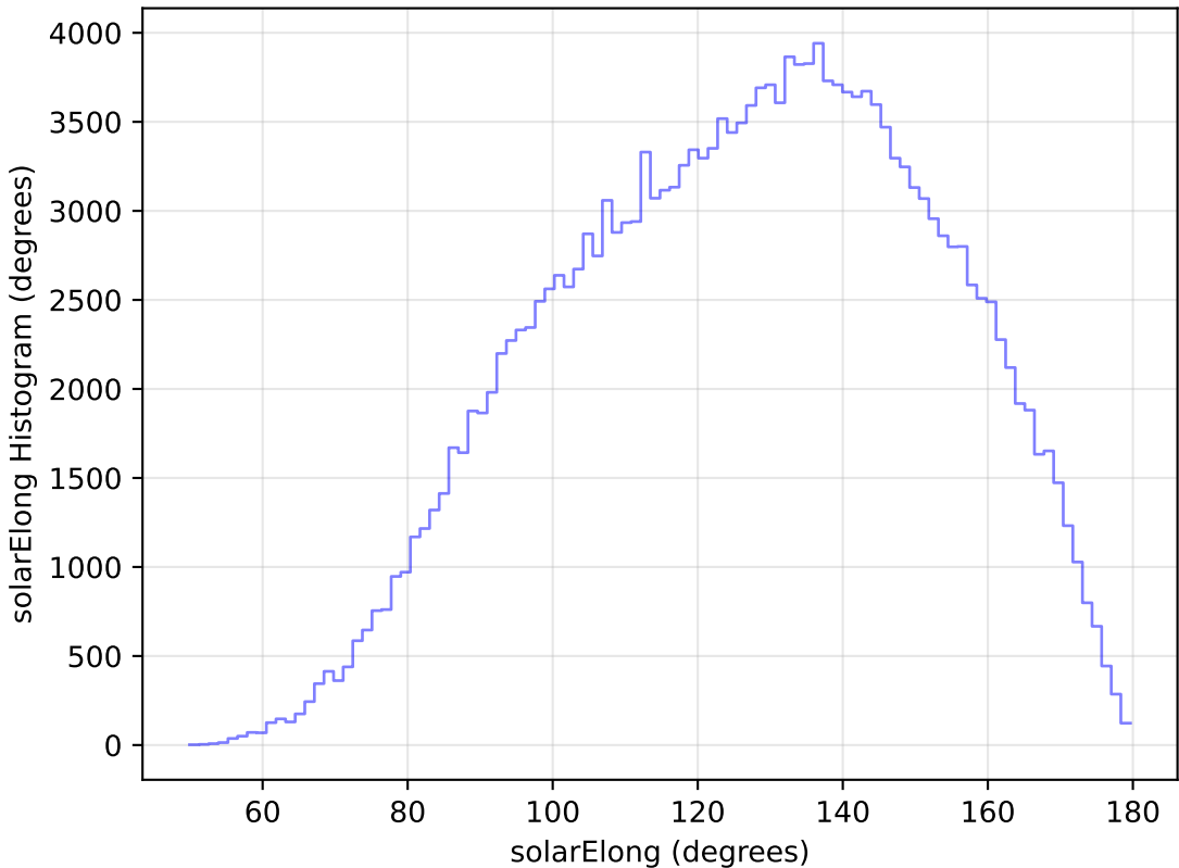
weather_cloudso2v3.4_10yrs All sky g band: solarElong Histogram
