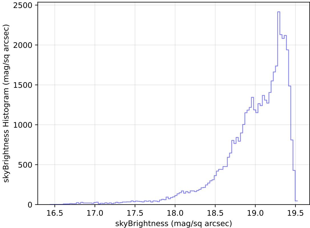
weather_cloudso2v3.4_10yrs Yr 1 z band: skyBrightness Histogram
