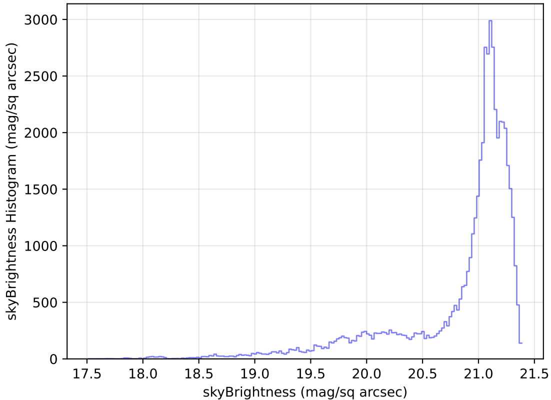
weather_cloudso2v3.4_10yrs Yr 1 r band: skyBrightness Histogram
