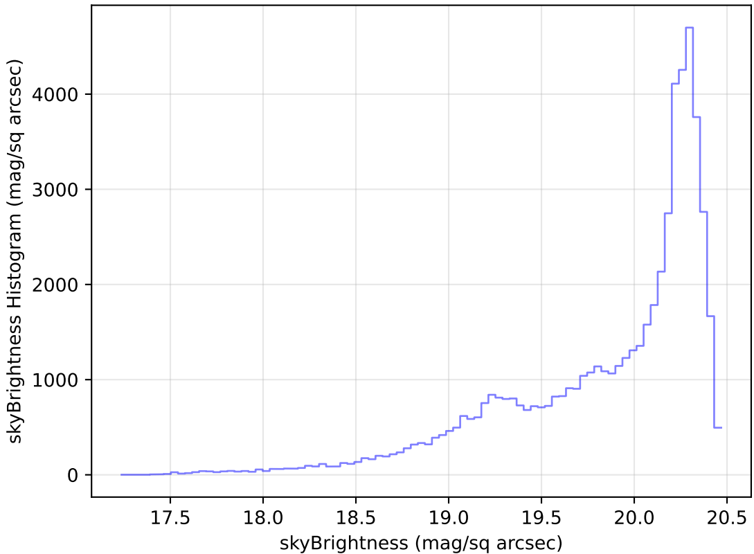
weather_cloudso2v3.4_10yrs Yr 1 i band: skyBrightness Histogram
