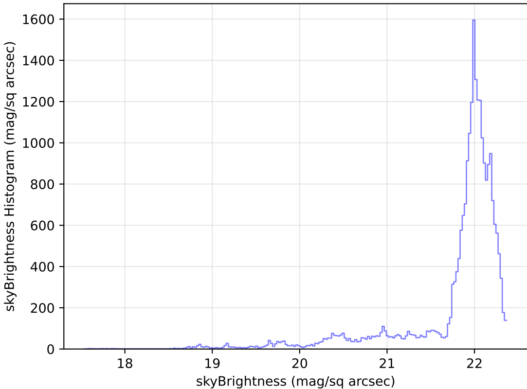
weather_cloudso2v3.4_10yrs Yr 1 g band: skyBrightness Histogram
