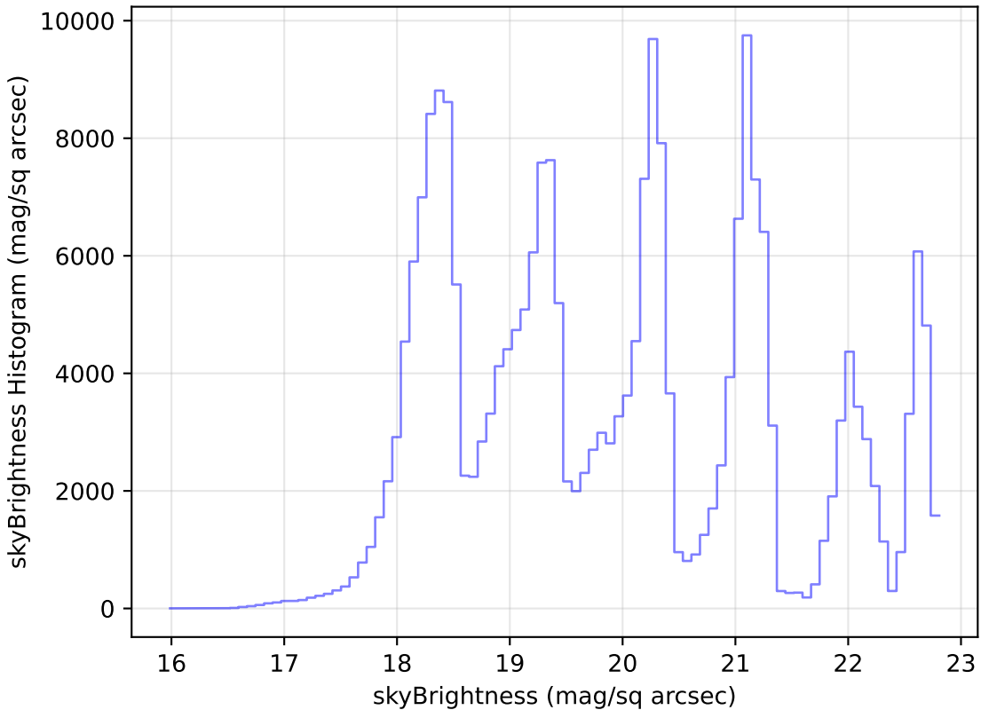
weather_cloudso2v3.4_10yrs Yr 1 all bands: skyBrightness Histogram
