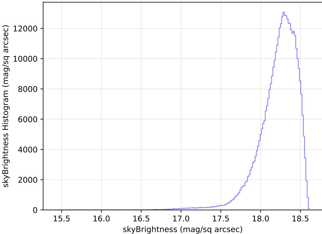
weather_cloudso2v3.4_10yrs WFD y band: skyBrightness Histogram
