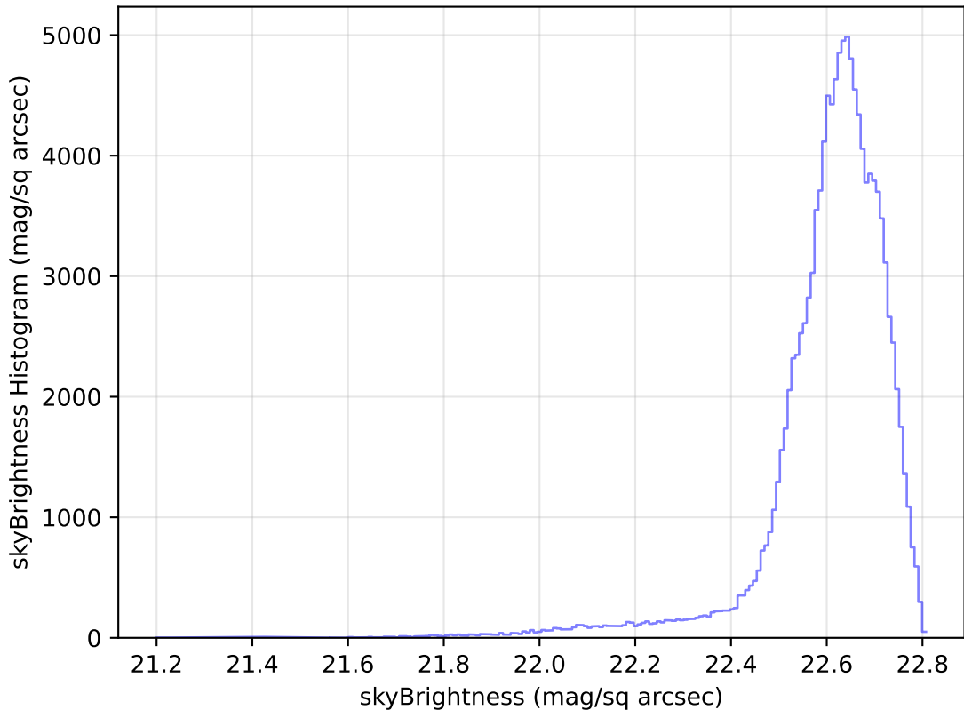
weather_cloudso2v3.4_10yrs WFD u band: skyBrightness Histogram
