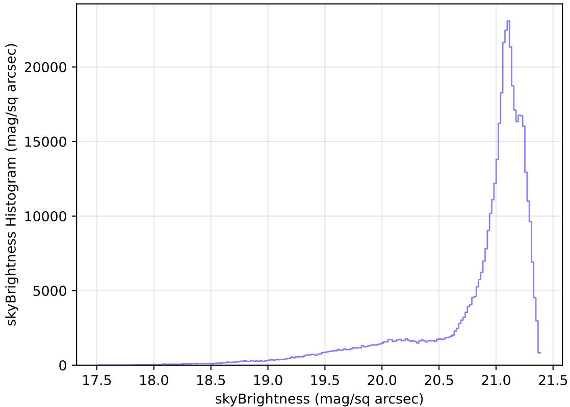
weather_cloudso2v3.4_10yrs WFD r band: skyBrightness Histogram
